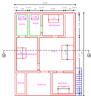
GROUND FLOOR PLAN (PROPOSED)
