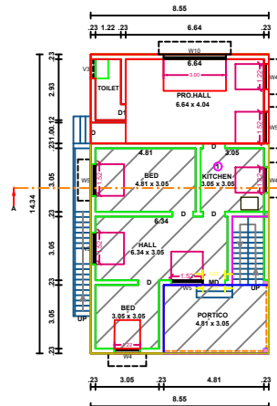
EXG. & PRO GROUND FLOOR PLAN
