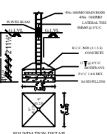
FOUNDATION DETAIL
