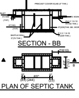
PLAN OF SEPTIC TANK
