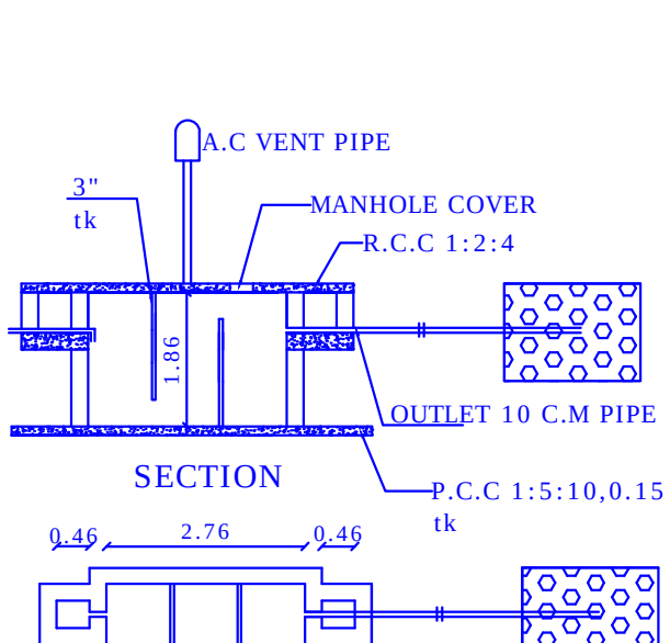
PLAN OF SEPTIC TANK & TRENCH
