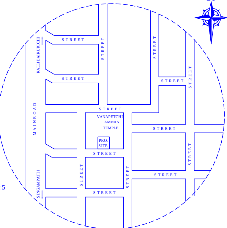
TOPO PLAN
