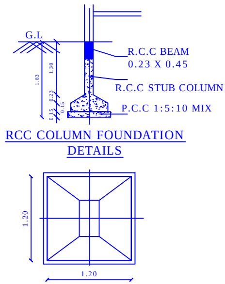
R.C.C FOOTING DETAILS
