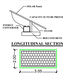
SOLAR SYSTEM
