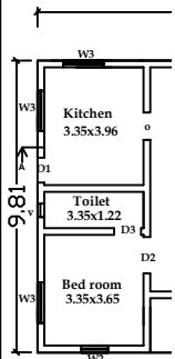
PROPOSED GROUND FLOOR PLAN
