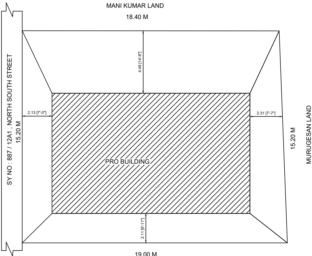
LOCATION PLAN
