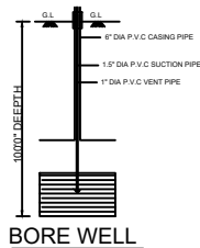
BORE WELL
