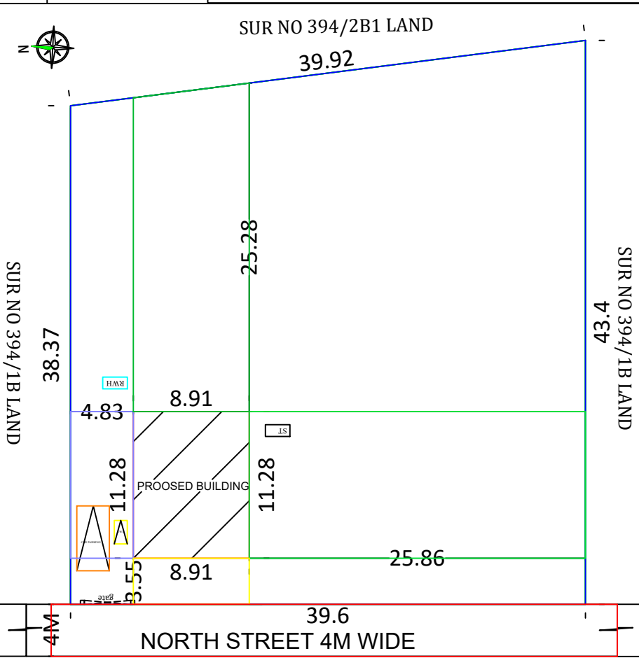
SITE PLAN 1:200 SCALE
