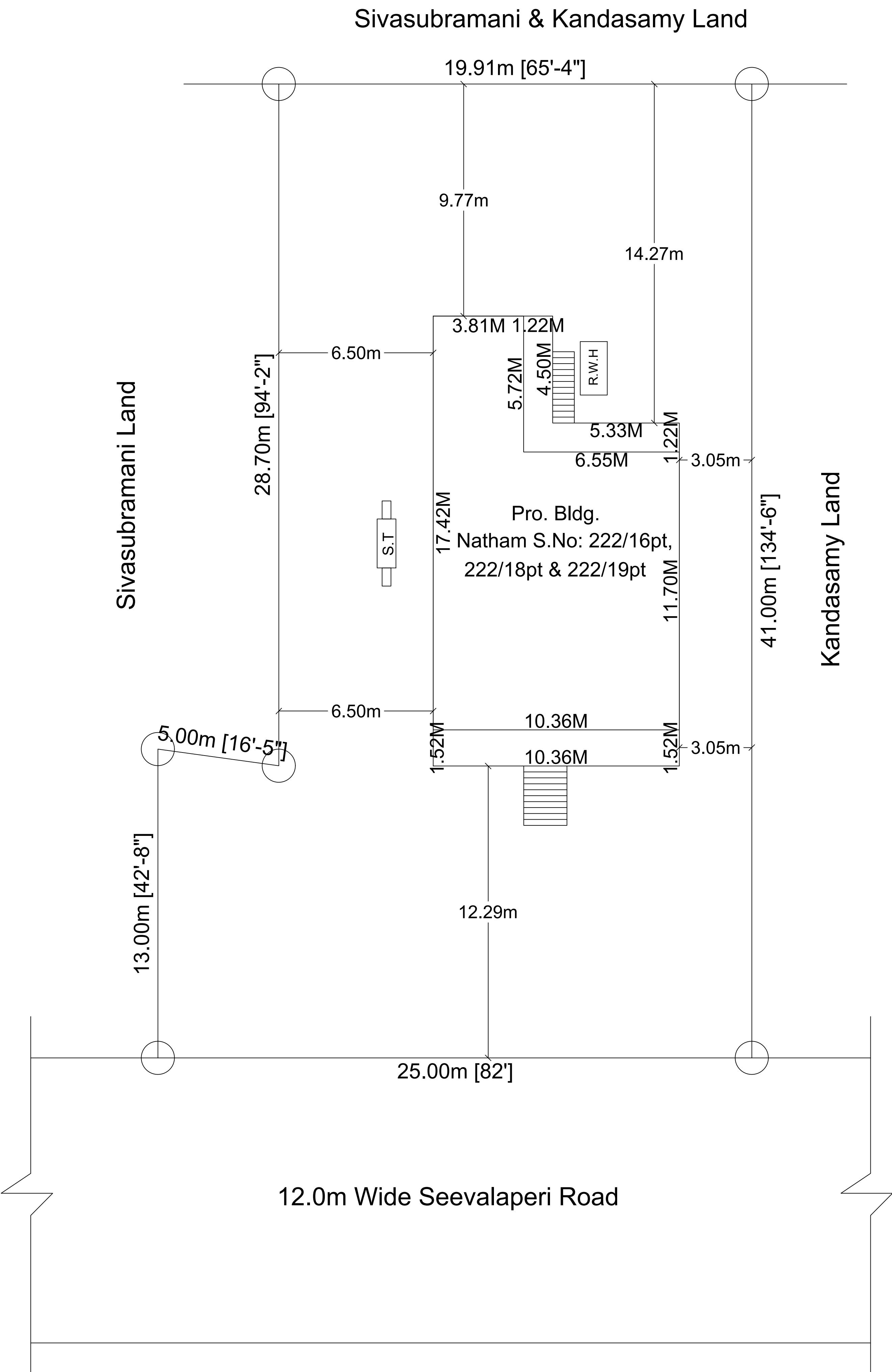
SITE PLAN
