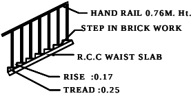
STAIR CASE DETAIL
