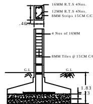
RCC COLUMN DETAILS
