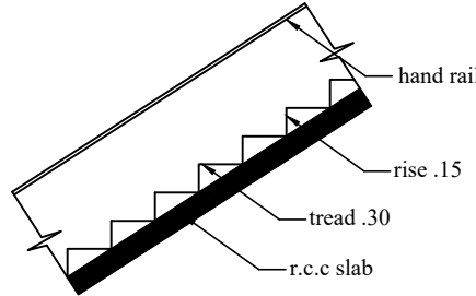
Stair
