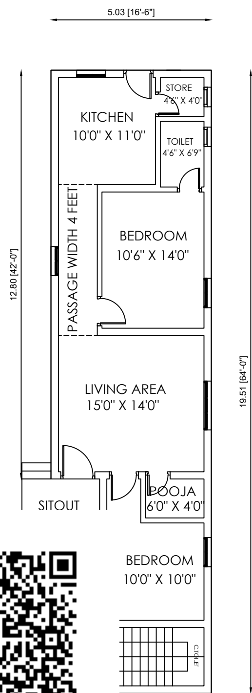
LOOR PLAN
