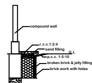
PLINTH BOUNDARY PERCOLATION PIT
