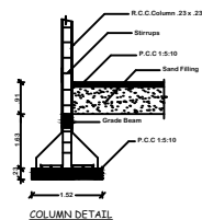
COLUMN DETAIL
