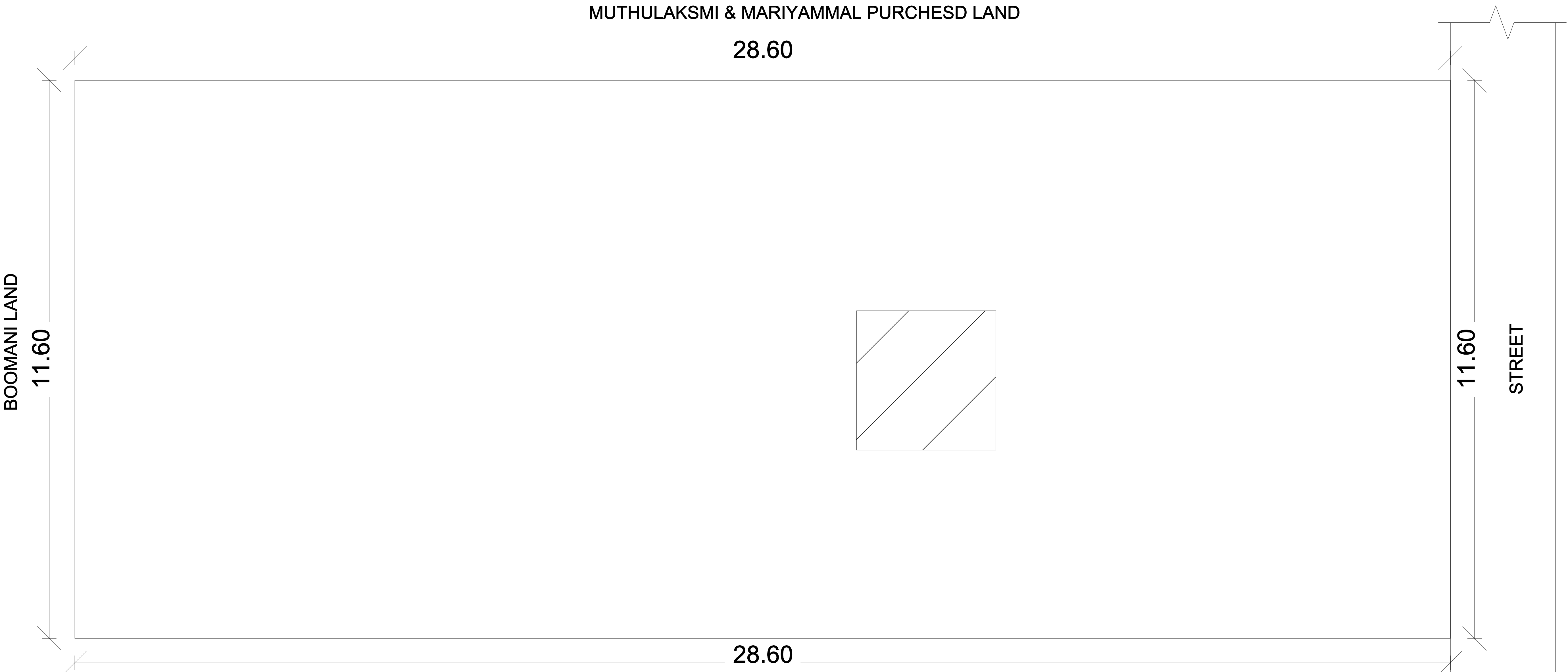
SITE PLAN
