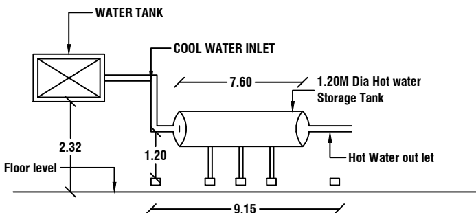
SOLAR WATER HEATING SYSTEM SWHS DETAILS
