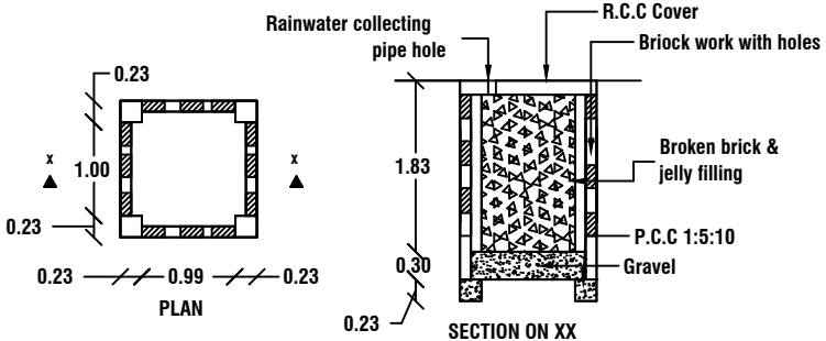
RAINWATER HARVEST WELL
