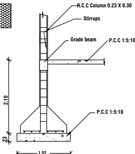
COLUMN DETAIL
