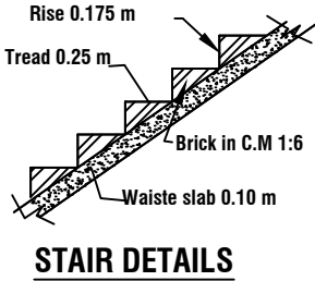
STAIR DETAILS
