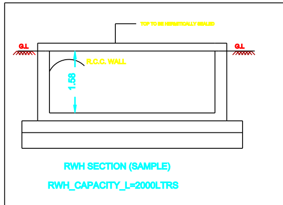
300mm x 300mm TRENCH DETAILS
