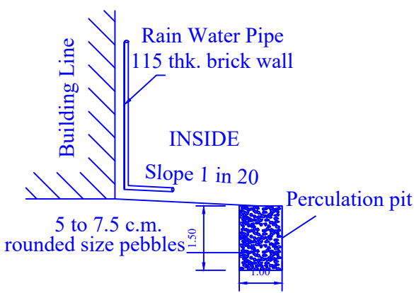
RAIN WATER HARVESTING SYSTEM
