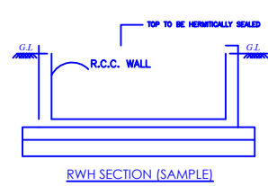
R.C.C. WALL SECTION (SAMPLE)
