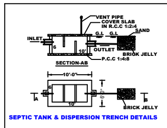
SEPTIC TANK & DISPERSION TRENCH DETAILS
