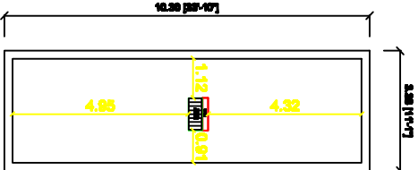
TERRACE FLOOR PLAN
