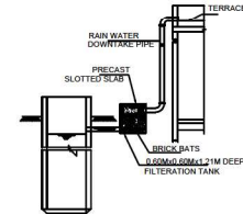
RAIN WATER HARVESTING SYSTEM
