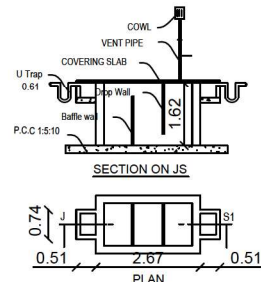
SECTION ON 'JS'
