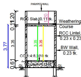
SECTION ON 'AB'
