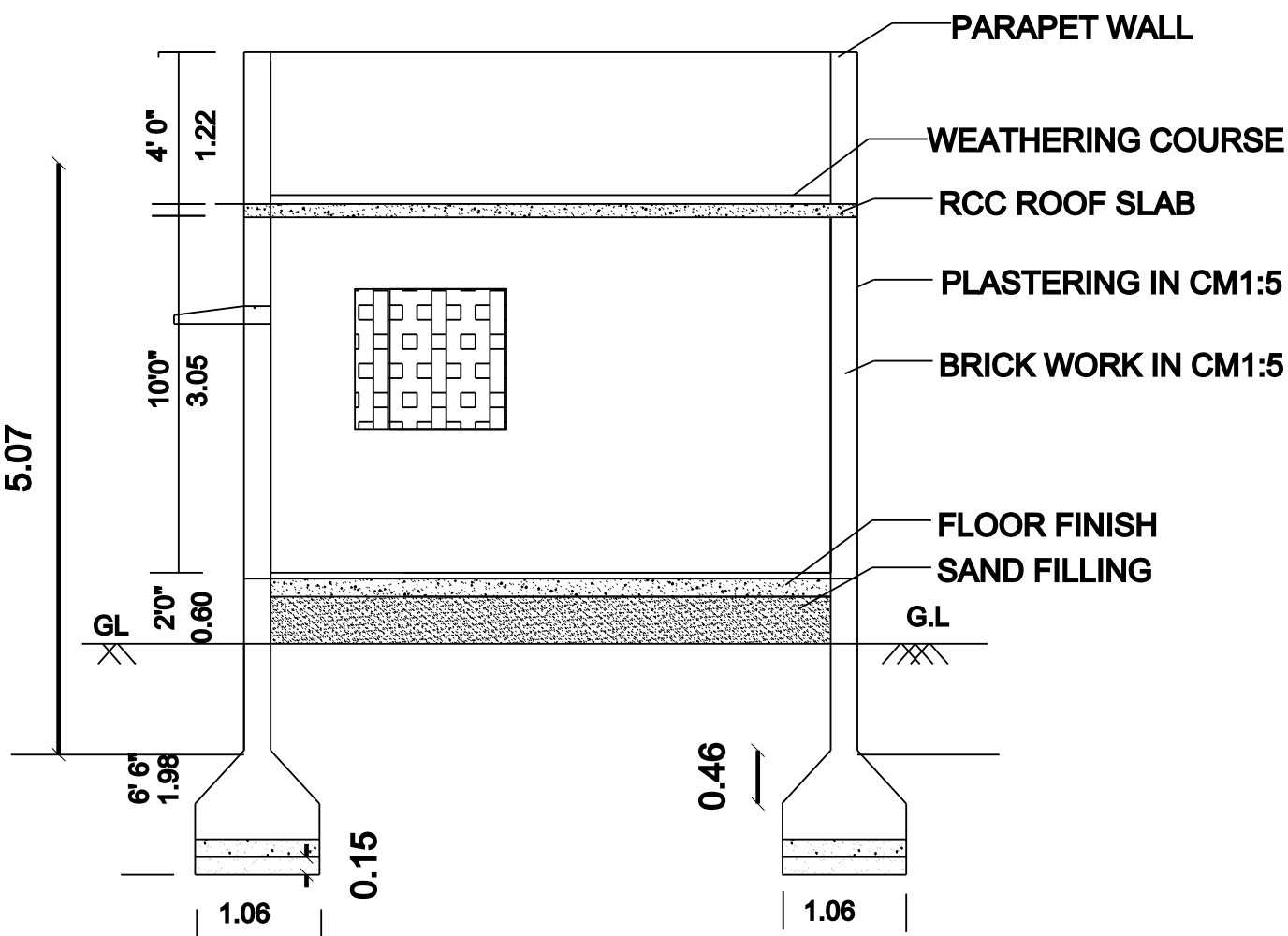
SECTION - AA'
