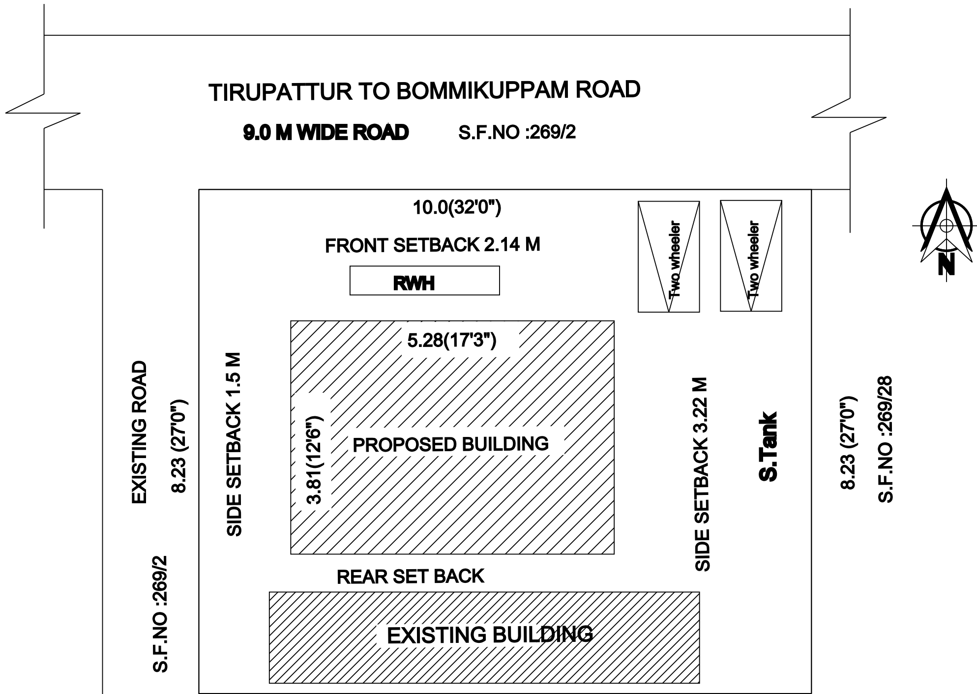
SITE PLAN
