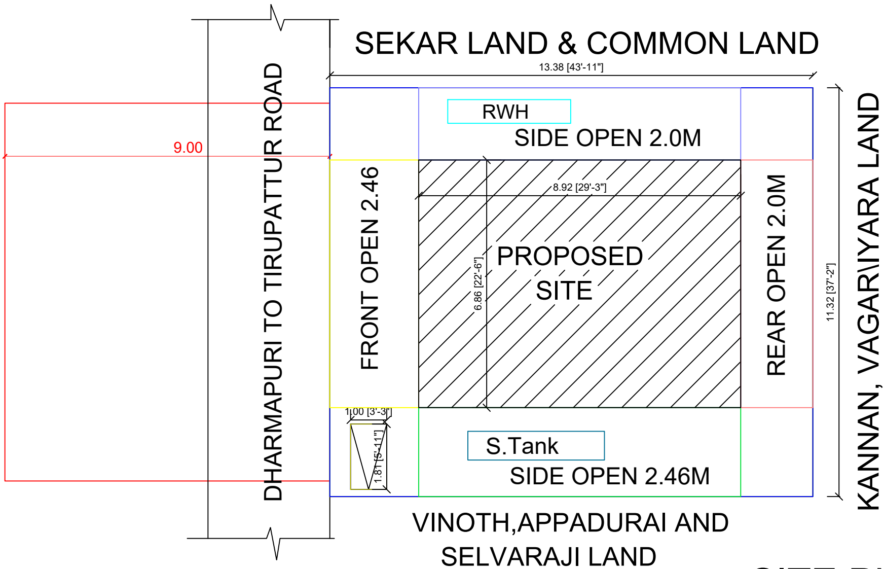
SITE PLAN
