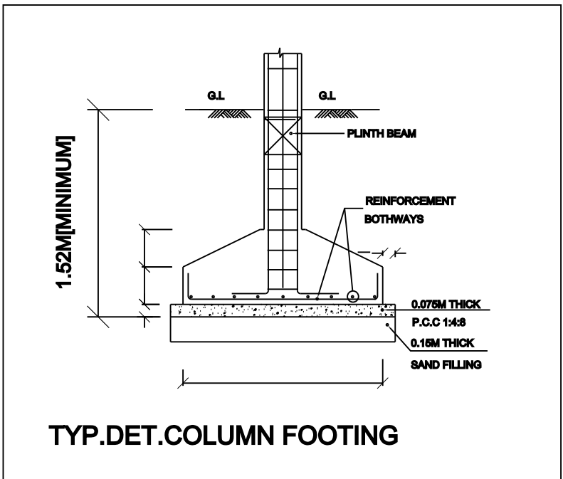
TYP.DET.COLUMN FOOTING
