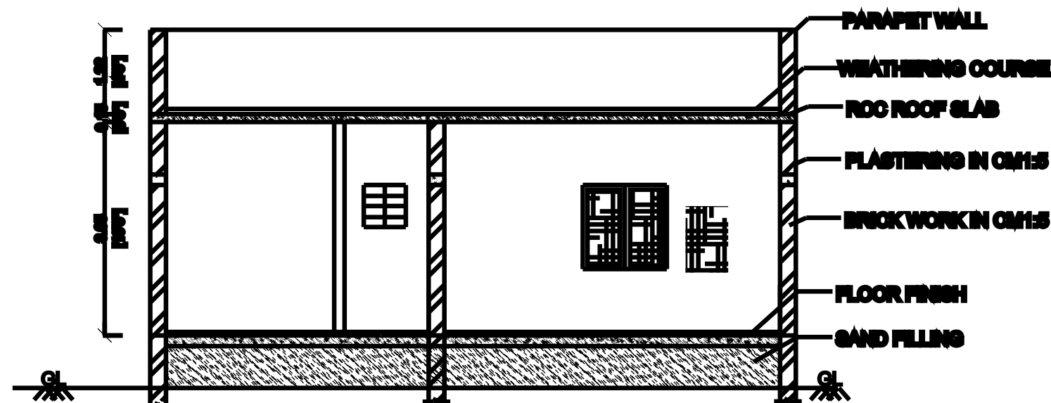
SECTION - AB'
