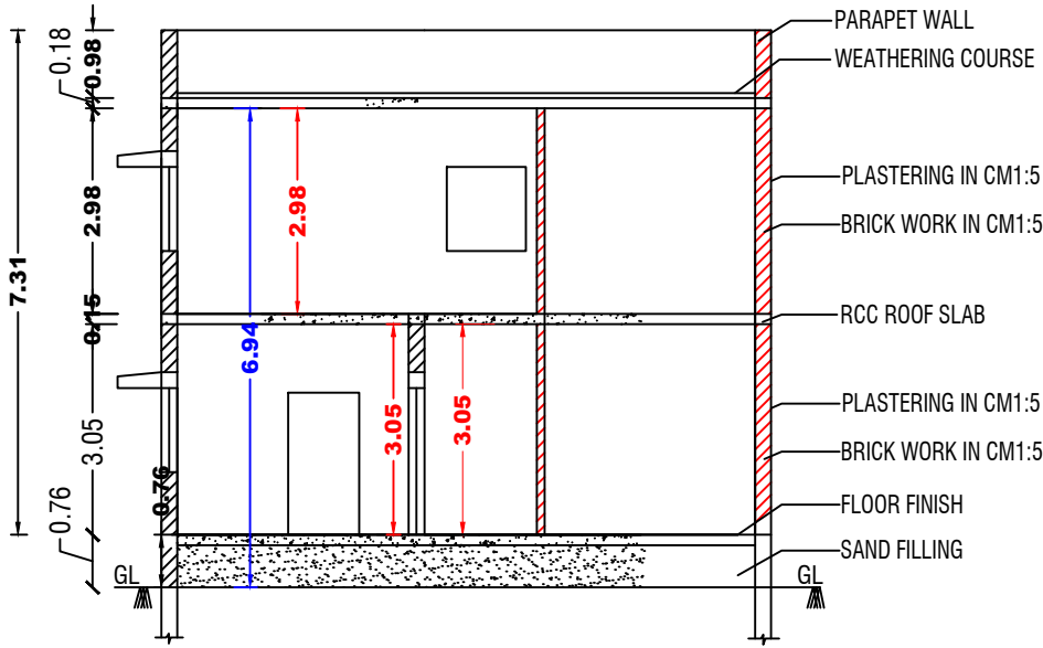
SECTION - AB'
