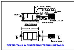
SEPTIC TANK & DISPERSION TRENCH DETAILS
