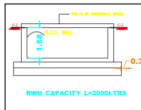
RWH CAPACITY L=2000LTRS
