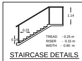
STAIRCASE DETAILS
