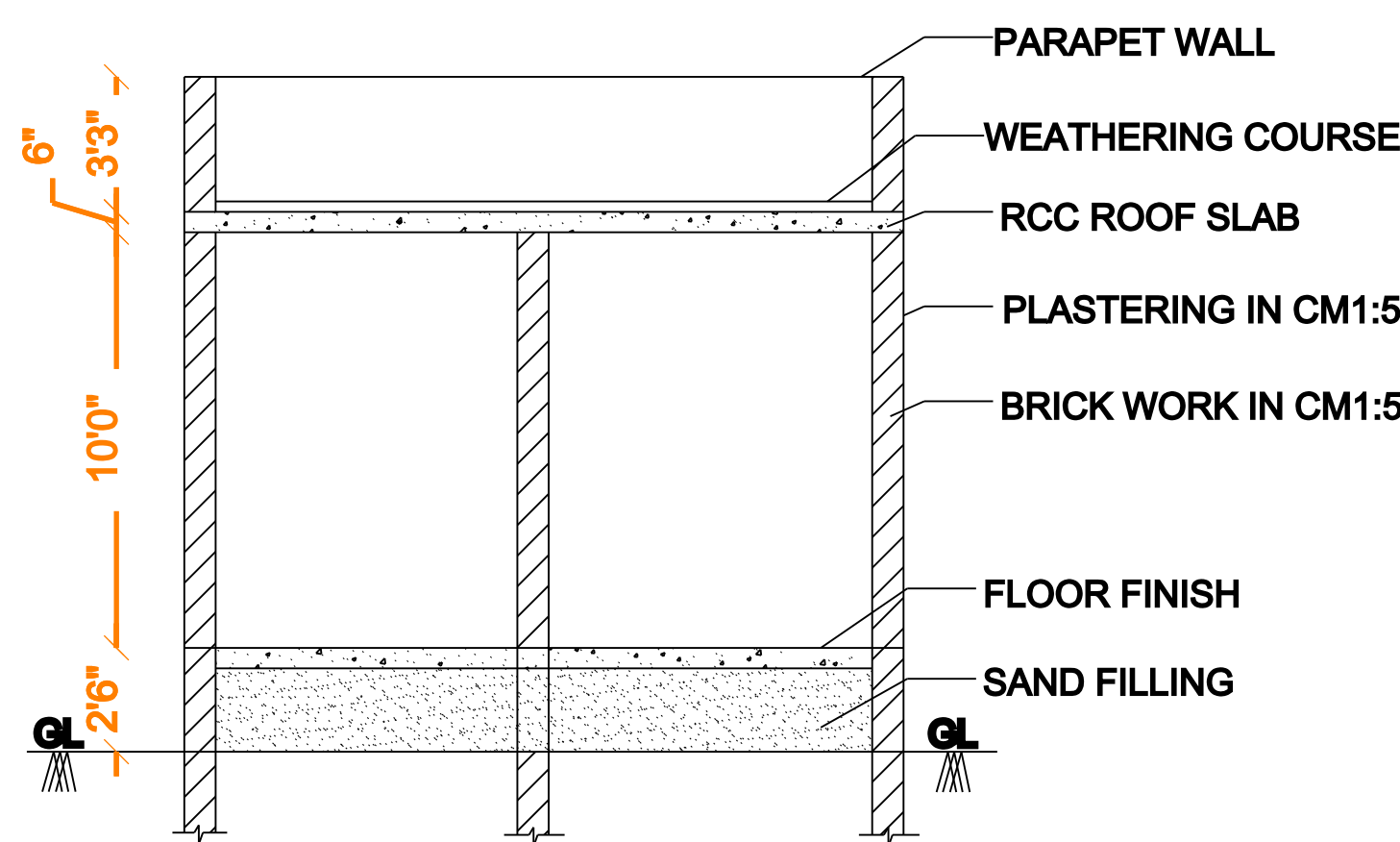
SECTION - AA'
