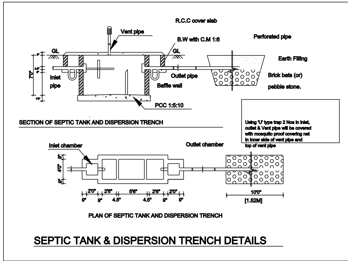
SEPTIC TANK & DISPERSION TRENCH DETAILS
