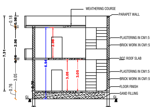
SECTION - AB'
