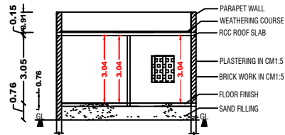
SECTION - AB'
