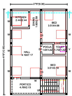
GROUND FLOOR PLAN (EXISTING BUILDING)
