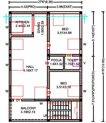
FIRST FLOOR PLAN (EXISTING & PROPOSED BUILDING)
