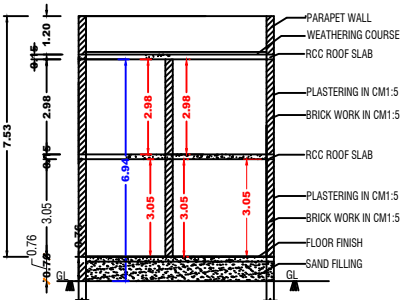
SECTION - AB'
