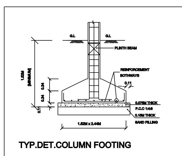
TYP.DET.COLUMN FOOTING
