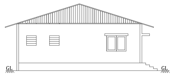
SOUTH SIDE ELEVATION
