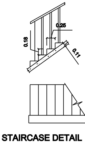
STAIRCASE DETAIL
