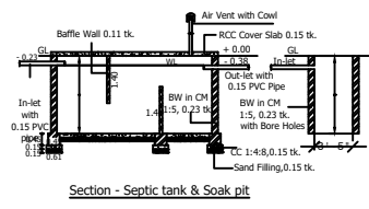
Section - Septic tank & Soak pit
