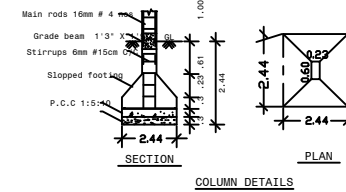
COLUMN DETAILS
