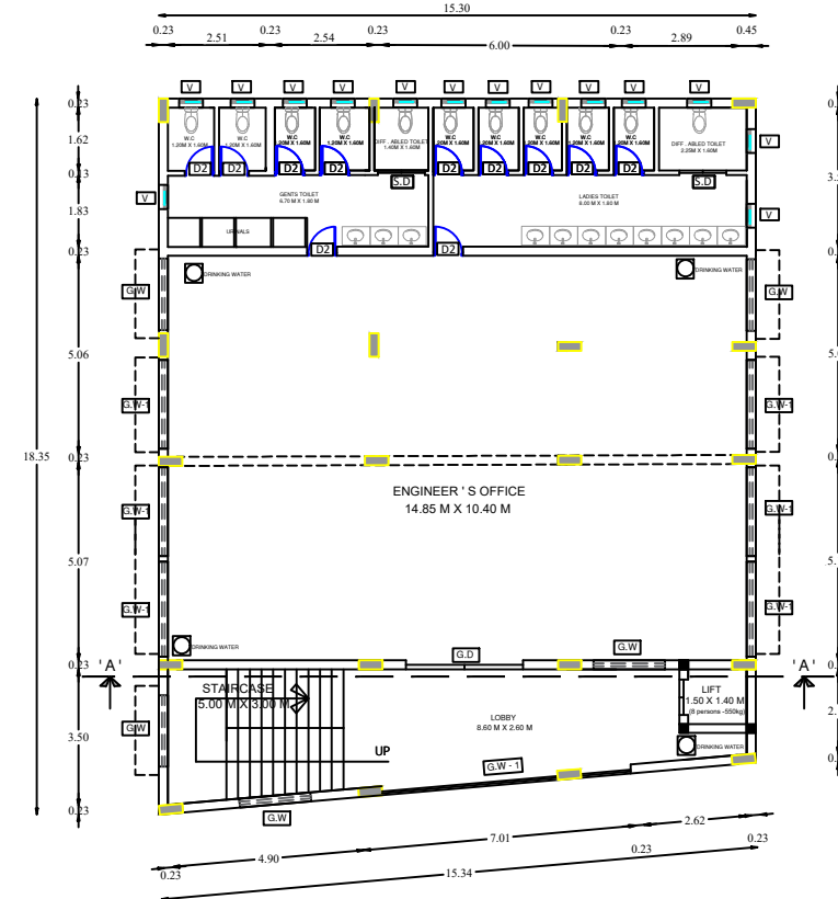
TYPICAL FLOOR PLAN (1st and 2nd Floors)
