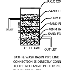
WASTE WATER RECYCLE UNIT
