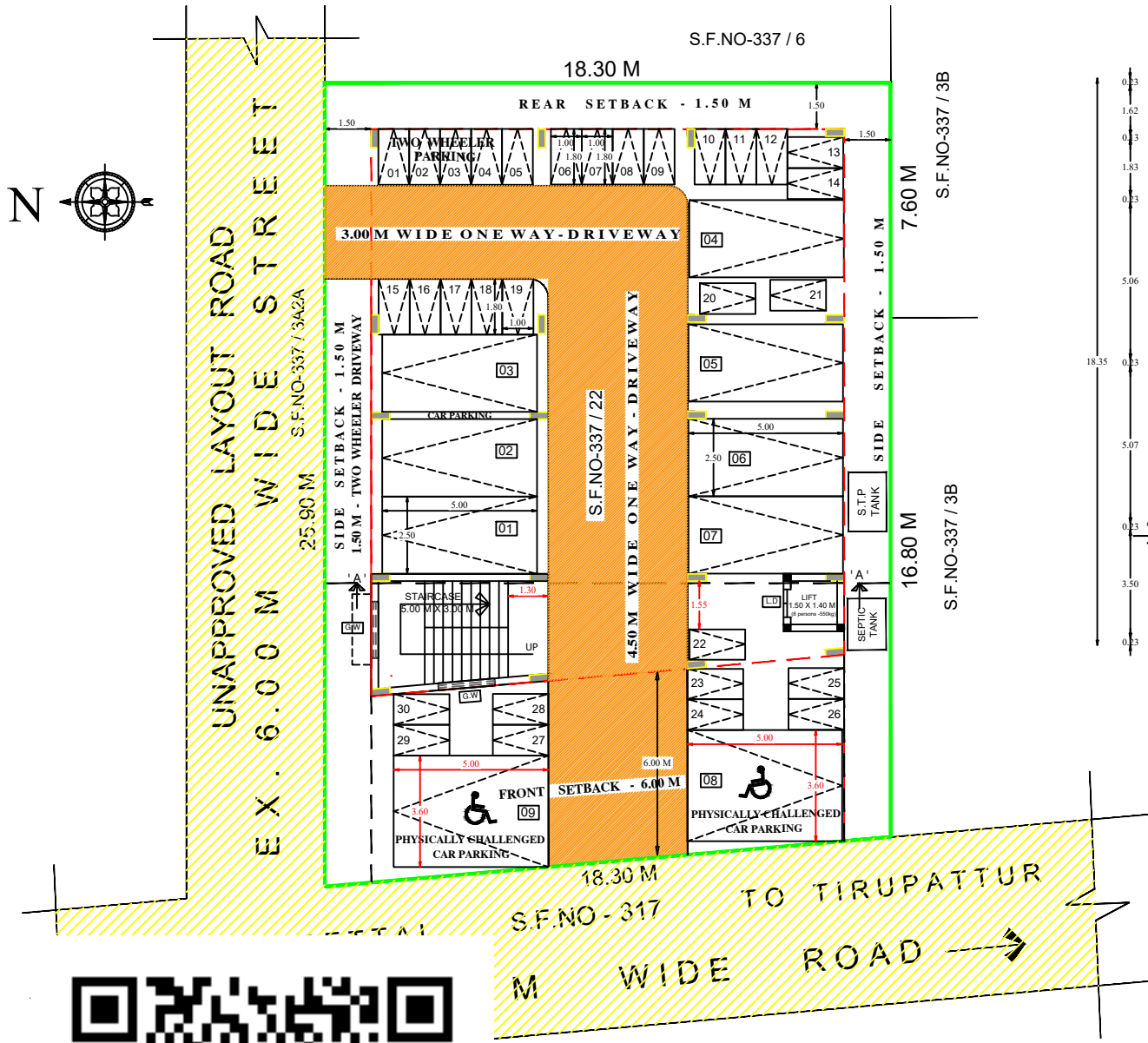
FLOOR PLAN
