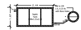
Plan - Septic tank & Soak pit
