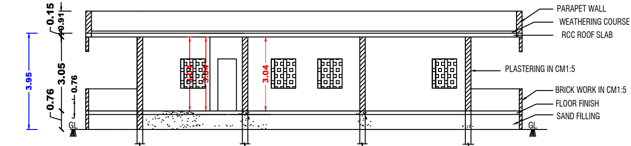
SECTION - AB'
