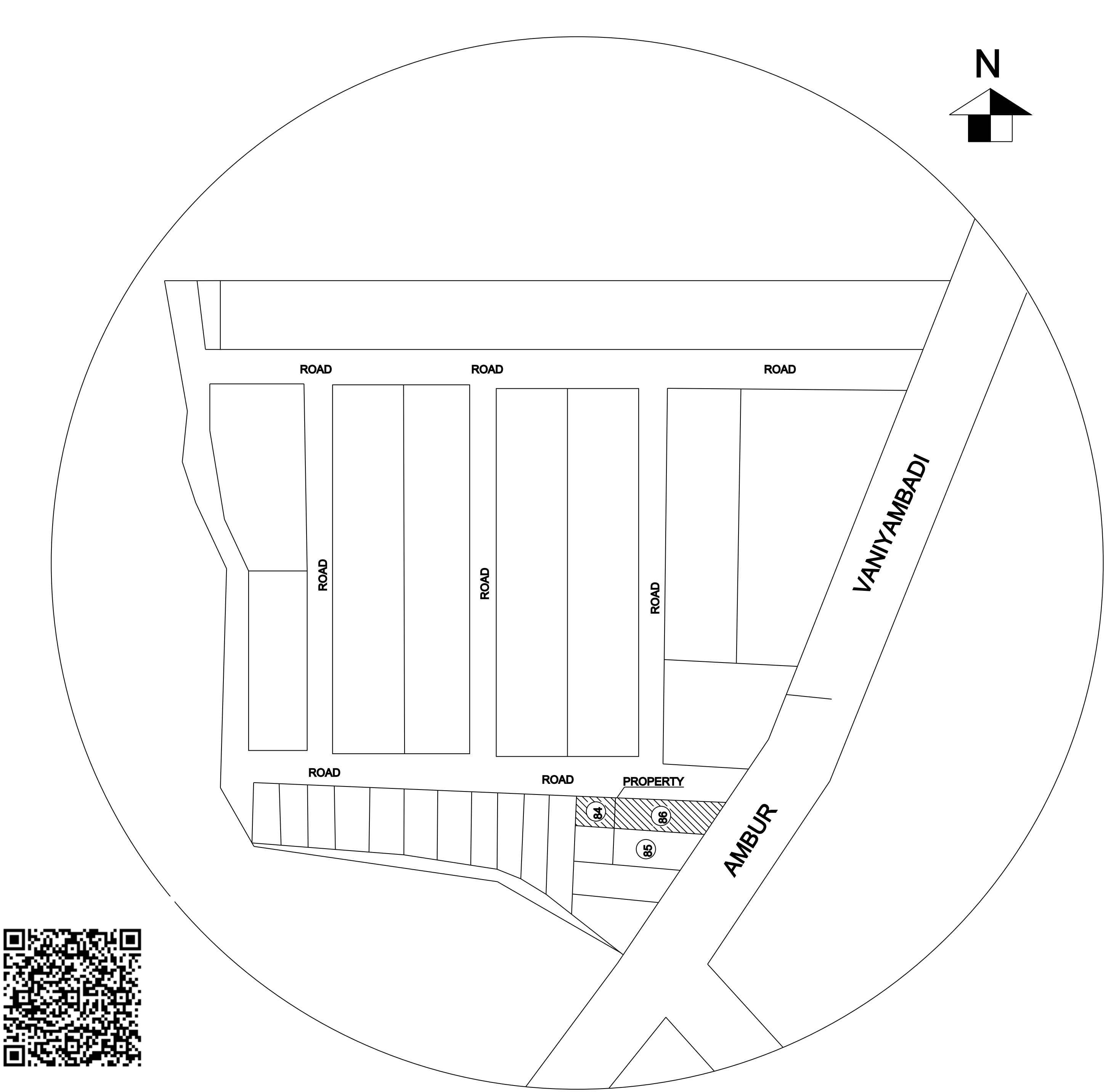
TOPO PLAN
