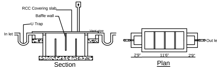
Septic tank with U Trap
