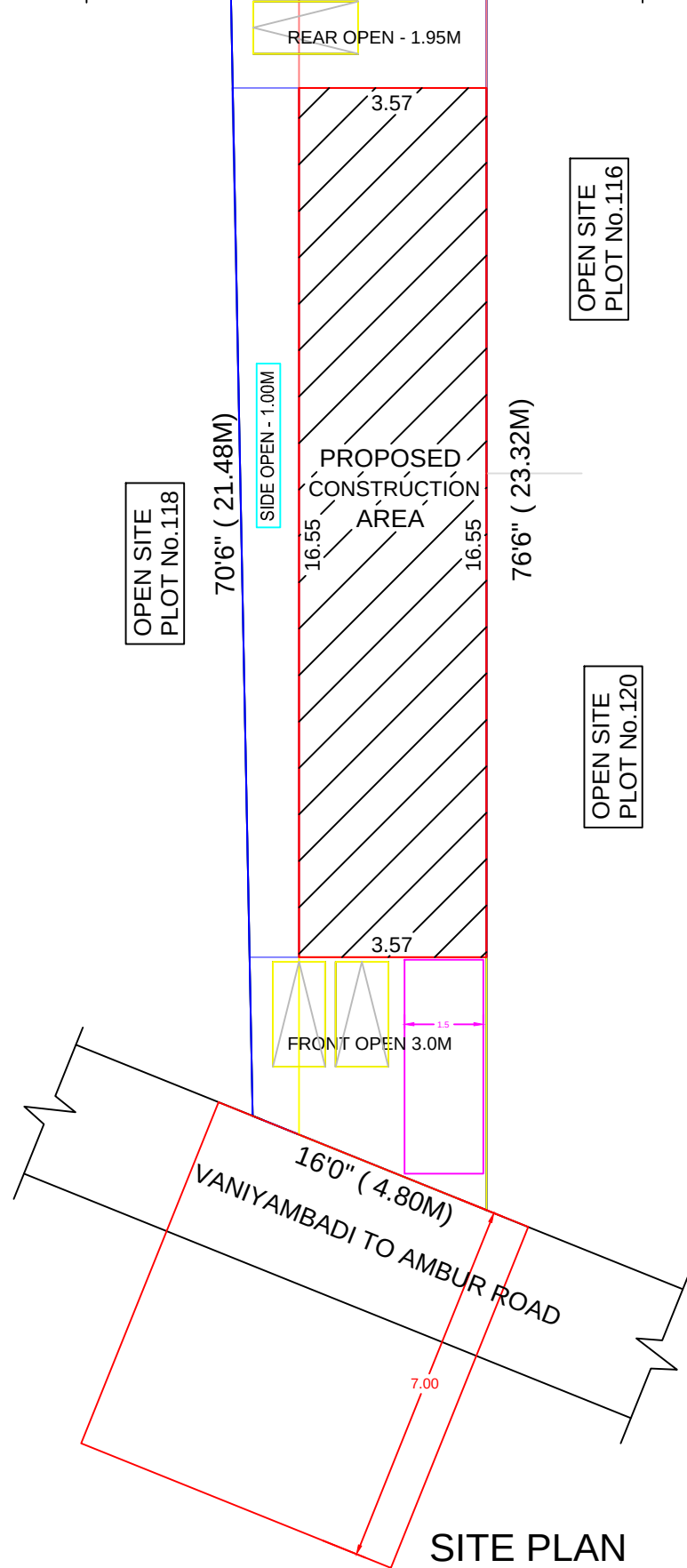
LAYOUT ROAD
