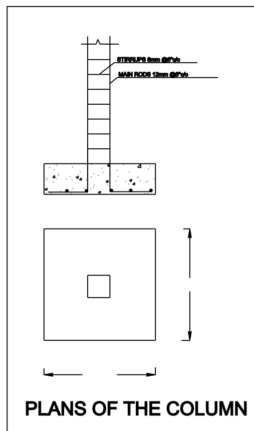
PLANS OF THE COLUMN
