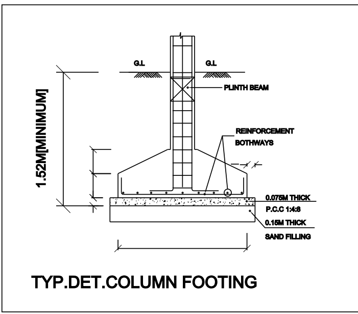
TYP.DET.COLUMN FOOTING
