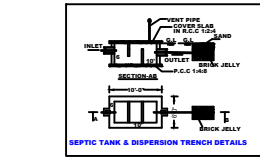
SEPTIC TANK & DISPERSION TRENCH DETAILS
