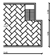
FLOOR PLAN
