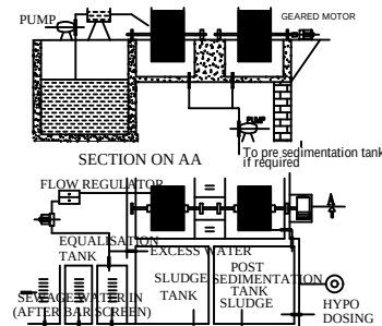
SEWAGE TREATMENT PLANT DETAILS
