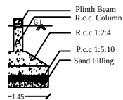
ROOTING DETAILS
