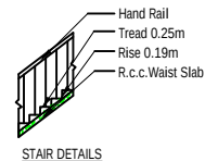
STAIR DETAILS
