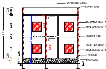
SECTION - AB'
