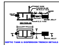
SEPTIC TANK & DISPERSION TRENCH DETAILS
