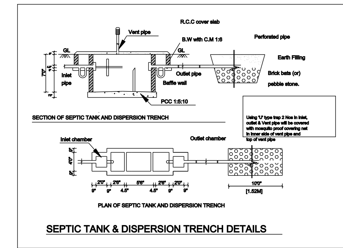
SEPTIC TANK & DISPERSION TRENCH DETAILS
