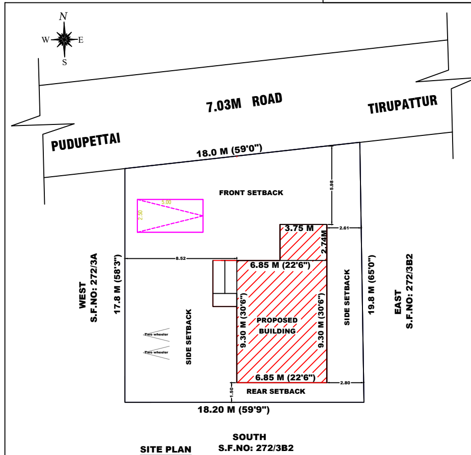
SITE PLAN
