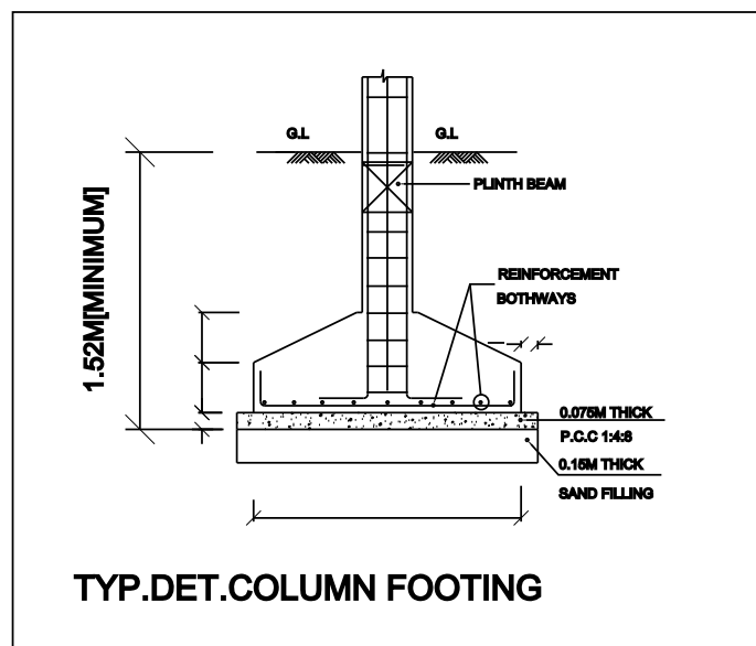
TYP.DET.COLUMN FOOTING
