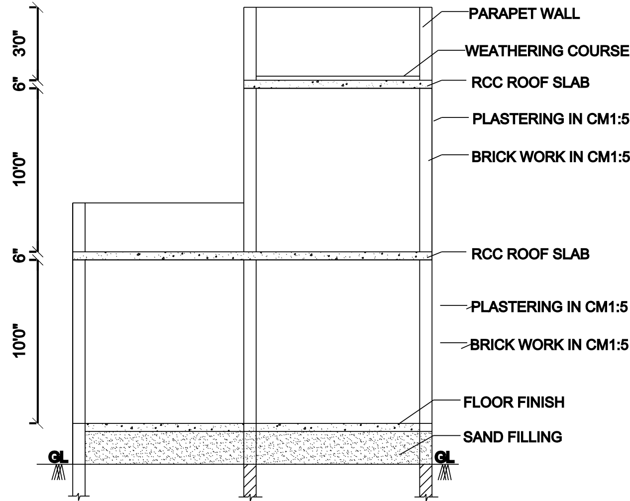
SECTION - AB'
