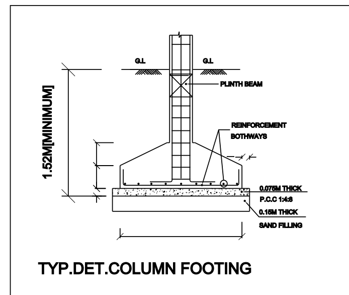
TYP.DET.COLUMN FOOTING
