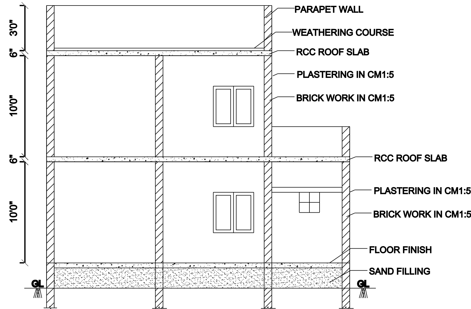
SECTION - AB'
