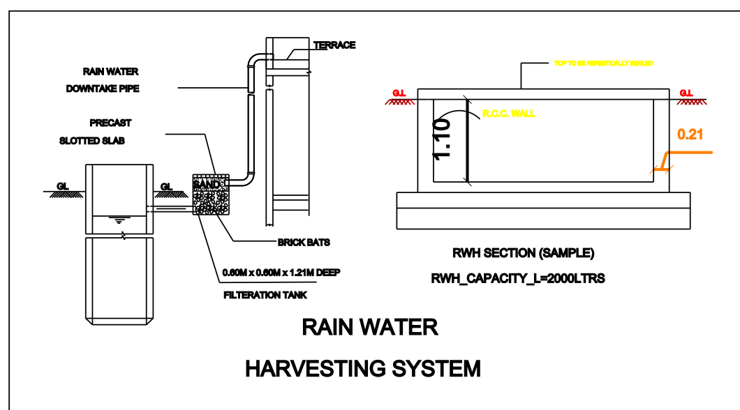
RAIN WATER HARVESTING SYSTEM
