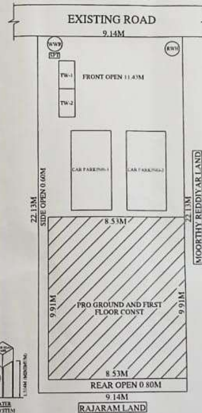
SITE PLAN
